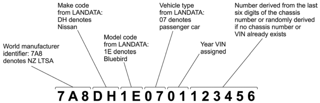
Figure 1-1-1. Structure of a VIN issued by NZTA
