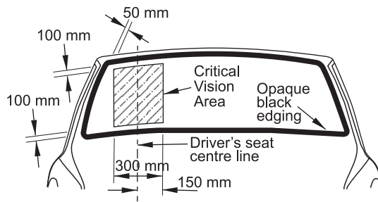
Figure 5-1-1. Windscreen critical vision area (CVA)
